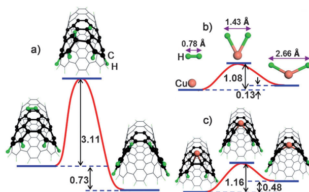
Figure 1. a) Unzipping of a SWNT with a hydrogen molecule, b) Cu-atom-catalyzed H–H bond breaking, and c) Cu-atom-catalyzed C–C bond breaking on the edge of a short (5,5) SWNT.
